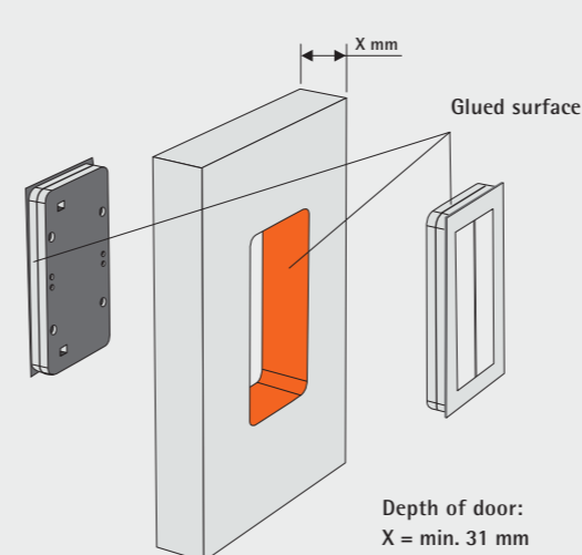
Typ L + S special (Handle on both sides glued)
