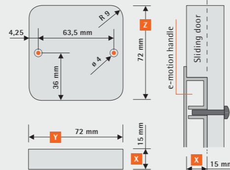
Typ S special (Handle on one side mounted)
