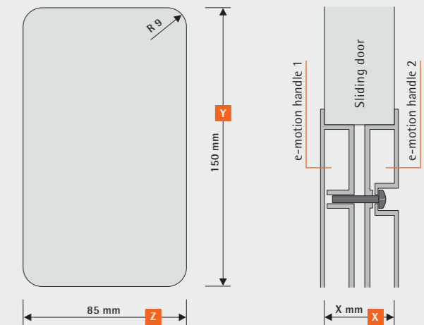
Typ L special+ (Handle on both sides mounted)
